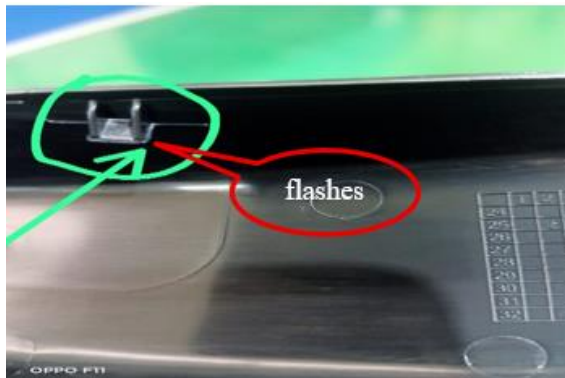
Gambar 4. Part Flashes
