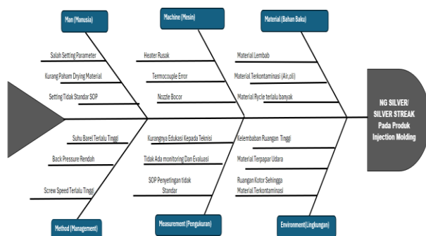
Gambar 5. Fishbone Diagram
