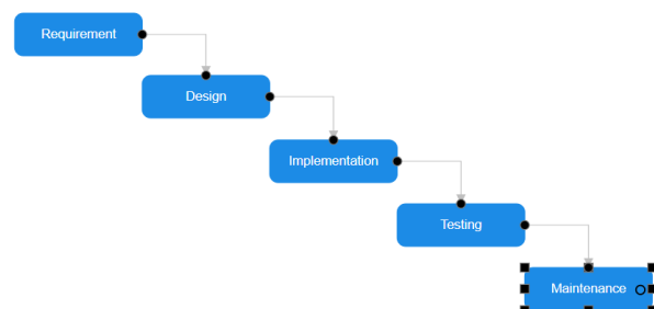
Gambar 1. Tahapan Waterfall
