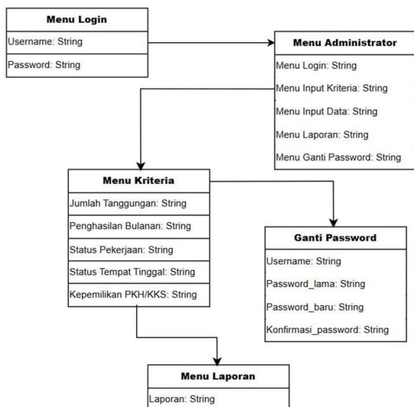
Gambar 6. Class Diagram
