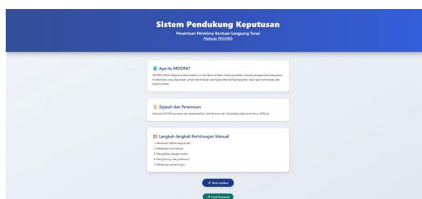
Gambar 8. Halaman Dashboard
