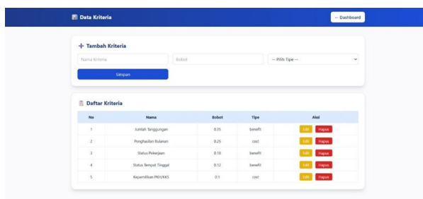
Gambar 9. Halaman Kriteria
