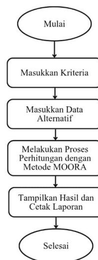
Gambar 4. Flowchart Sistem
